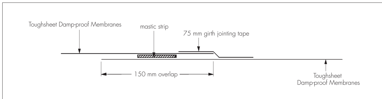
Figure 1 Mastic tape joint
